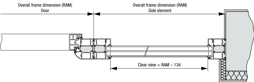
Frame variants, Thermo65
