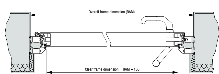
Horizontal view of door, Thermo65
