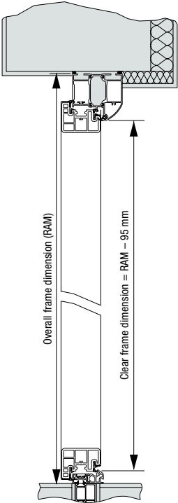
Vertical view of door, Thermo65
