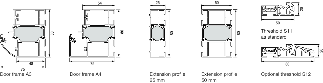
Frame variants, Thermo65
